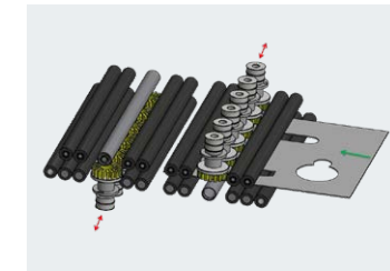
DiscMaster SF 1/1
